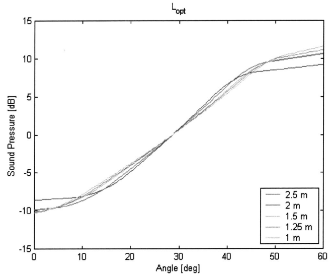
FIG. 8. \ell_{\text{opt}} 's in the working region ( 0^\circ - 60^\circ ) for several stereo base distances.
